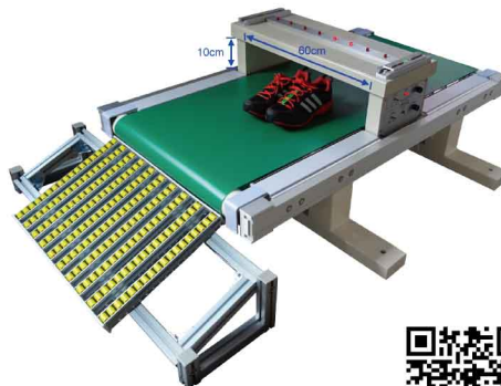
置生產線檢針機 INS-330K-60XX Low Profile Platform
